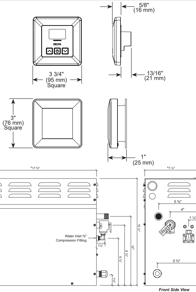
Steam Generator Specification Chart
